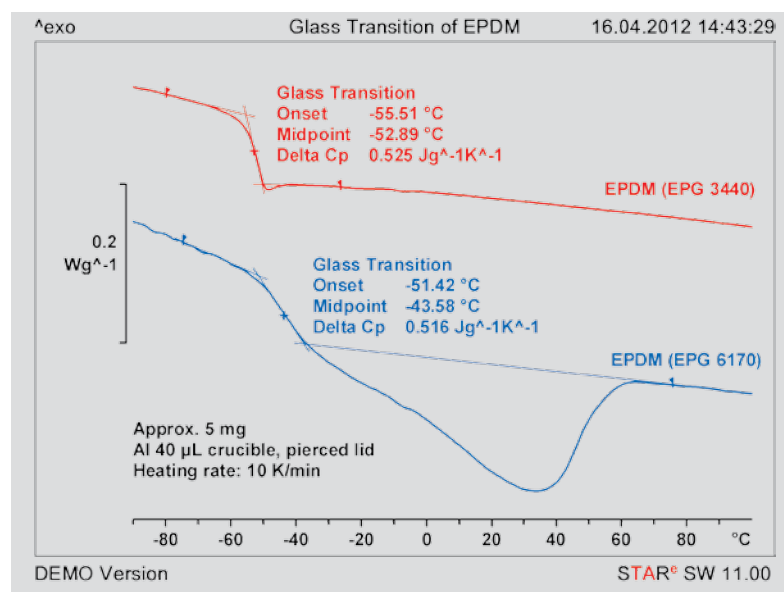
Figure 32. Determination of the glass transition temperature of two samples of unvulcanized EPDM with different ethylene contents.
