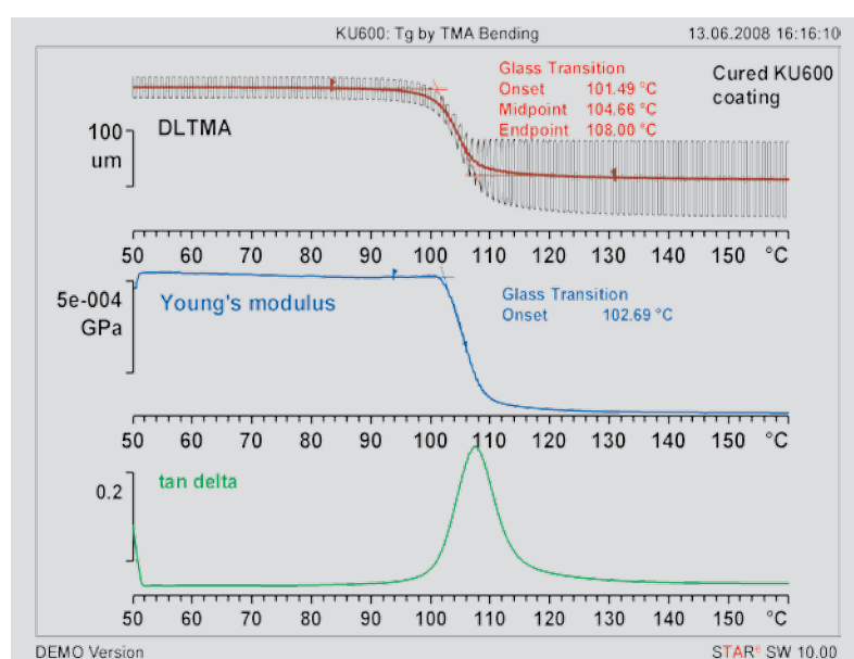
Figure 27. DLTMA measurement of a cured KU600 coating.
