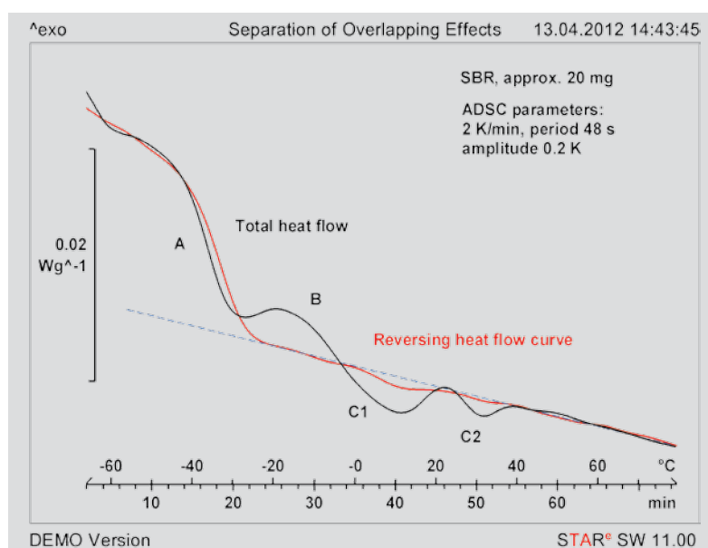
Figure 35. Separation of overlapping effects of unvulcanized SBR using ADSC.
