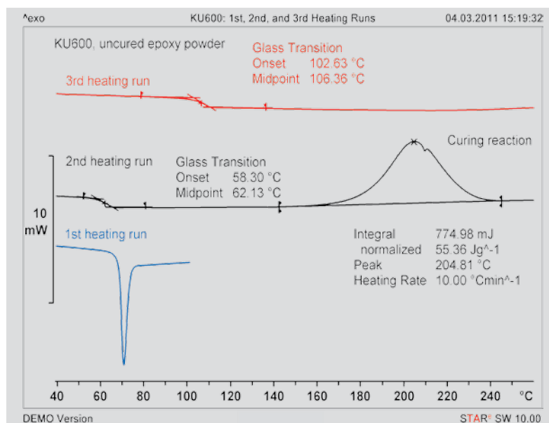
Figure 18. KU600: DSC experiment at a heating rate of 10 K/min showing the first, second and third heating runs.
