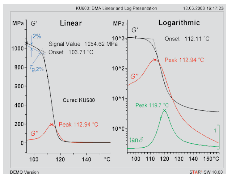
Figure 29. DMA measurement of KU600 from 90 to 160 °C, in linear and logarithmic ordinate presentation.
