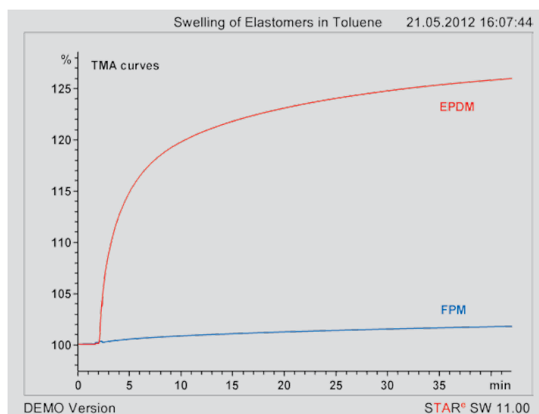
Figure 43. Swelling measurements of cylindrical EPDM and FPM elastomer samples (diameter 2 mm, thickness 2.5 mm) in toluene at 30 °C.
