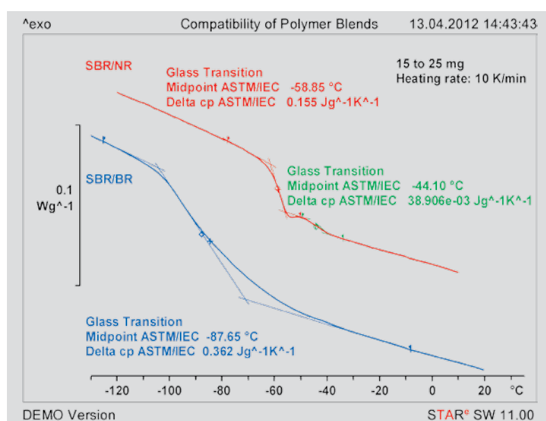
Figure 33. DSC analysis of the compatibility of two SBR polymer blends.
