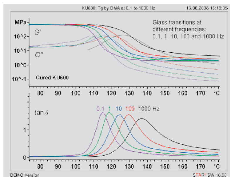
Figure 30. DMA measurement of KU600 at different frequencies to demonstrate the frequency dependence of the glass transition.
