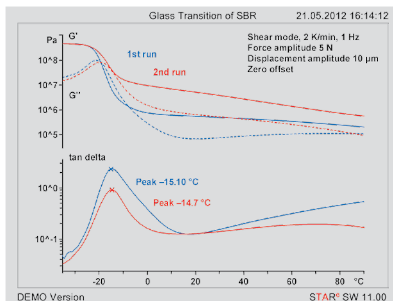
Figure 44. The curves show the first and second heating runs of a cylindrical sample of unvulcanized SBR (diameter 6.5 mm, thickness 0.7 mm) without filler, measured by DMA in the shear mode.
