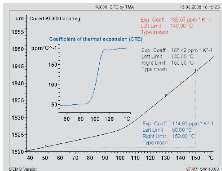
Figure 26. Determination of the coefficient of thermal expansion (CTE) of cured KU600 using the second heating run.
