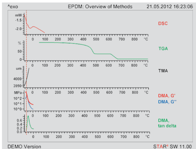
Figure 48. Overview of effects and comparison of results. The glass transition temperature is shown by a vertical dashed line.
