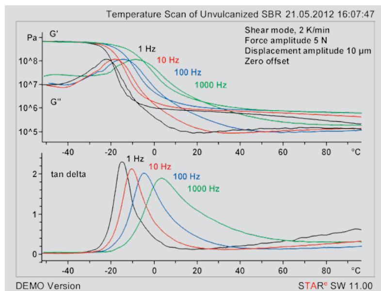
Figure 45. Temperature scan of a cylindrical sample of unvulcanized SBR (diameter 4 mm, thickness 1.0 mm) without filler at 1, 10, 100 and 1000 Hz.
