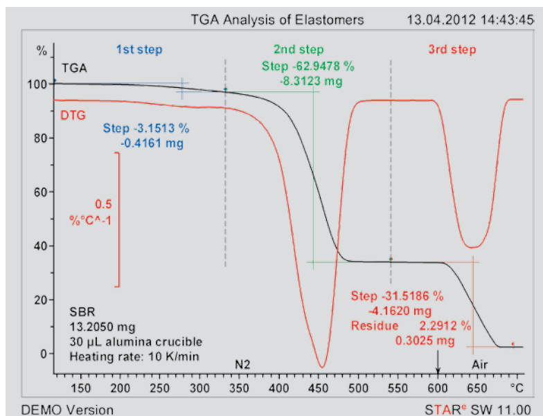
Figure 38. TGA analysis of an SBR elastomer.
