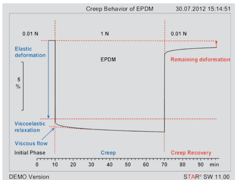
Figure 41. TMA curves showing the creep and creep recovery behavior of a rectangular EPDM sample (width 3.5 mm, length 3.5 mm, thickness 1.5 mm) measured at 30 °C.
