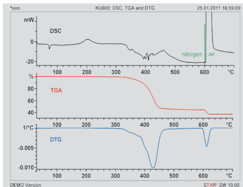
Figure 25. TGA/DSC 1 curves of KU600 epoxy powder measured from 30 to 700 °C at a heating rate of 20 K/min. The TGA curve (red) measures the loss of mass and the DSC curve (black) provides information about endothermic and exothermic effects.
