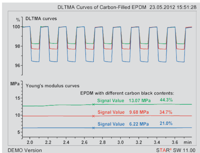
Figure 42. Determination of the Young's modulus of three rectangular EPDM samples (width 2 mm, length 2 mm, thickness 1.5 mm) with carbon black contents of 21.0, 34.7 and 44.3% by DLTMA.
