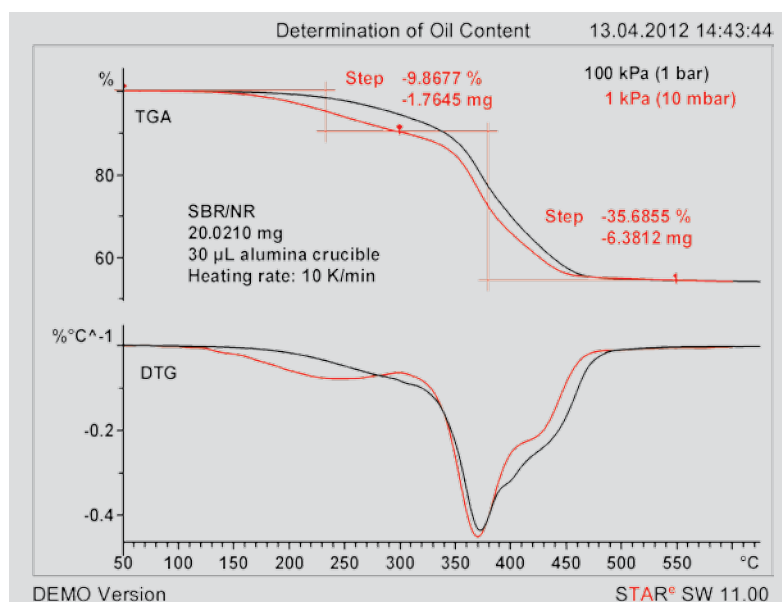
Figure 39. Determination of the oil content of an SBR/NR elastomer using TGA at ambient pressure and reduced pressure.
