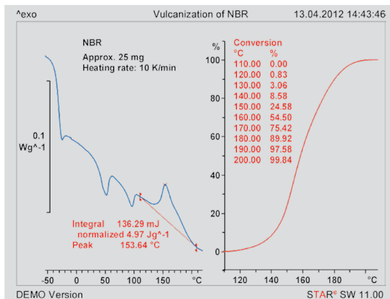
Figure 36. DSC measurement curve of an unvulcanized sample of NBR.
