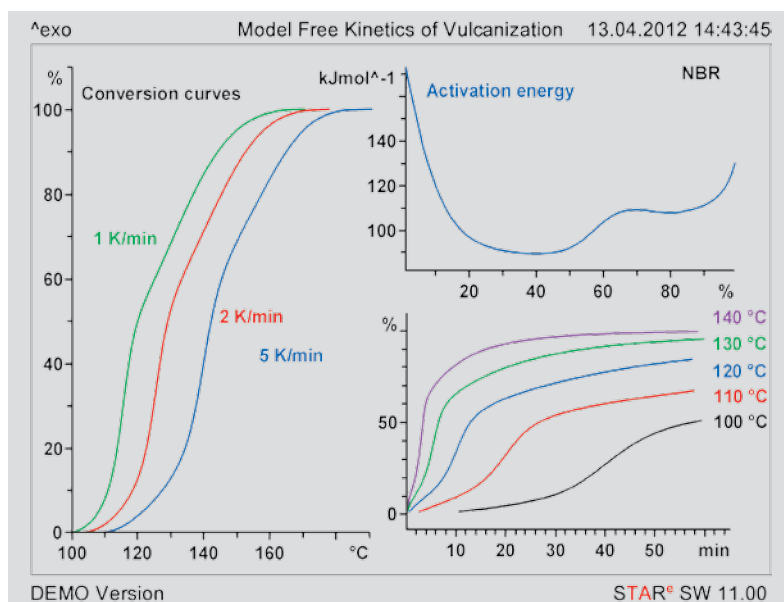
Figure 37. Model Free Kinetics of the vulcanization of NBR.
