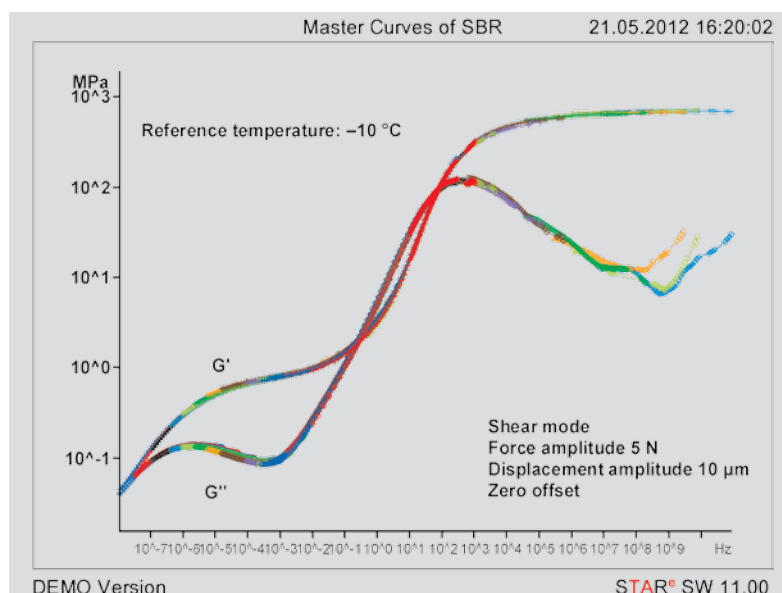
Figure 47. Master curves of the storage and loss moduli of a cylindrical sample of unvulcanized SBR without filler (diameter 4.00 mm, thickness 1.0 mm) at a reference temperature of -10\text{ }^{\circ}\text{C} measured in the shear mode.
