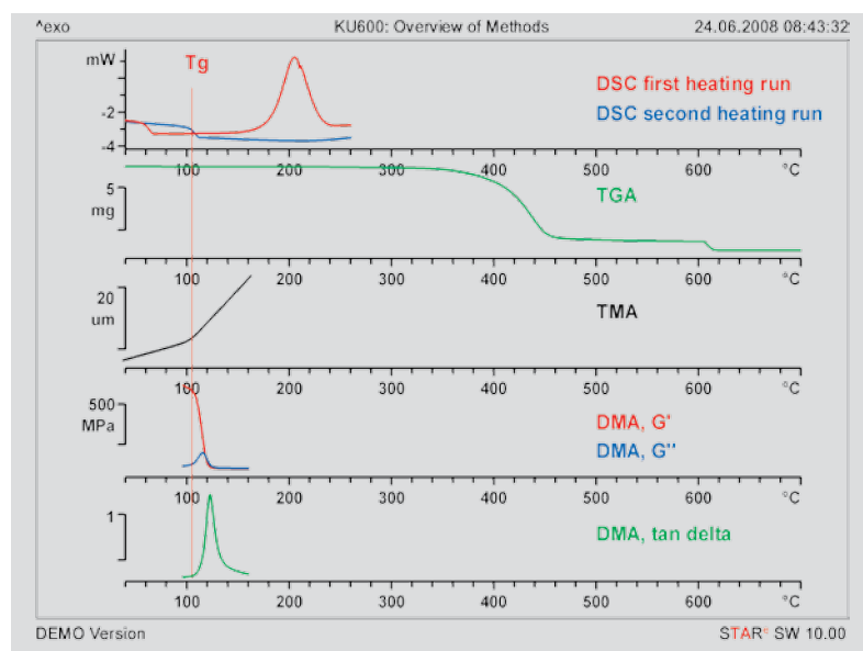
Figure 31. Overview of the effects and comparison of results.
