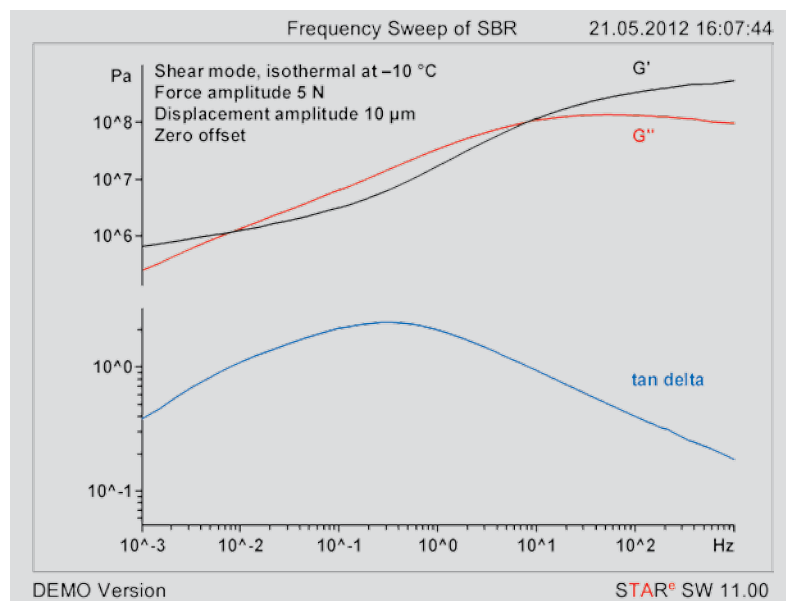
Figure 46. Frequency measurements of a cylindrical sample of unfilled SBR (diameter 5.0 mm, thickness 1.2 mm) vulcanized with 2 phr sulfur.
