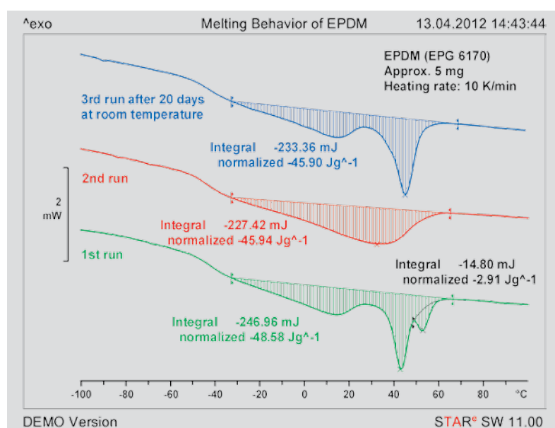
Figure 34. Influence of pretreatment on the melting of a sample of unvulcanized EPDM.
