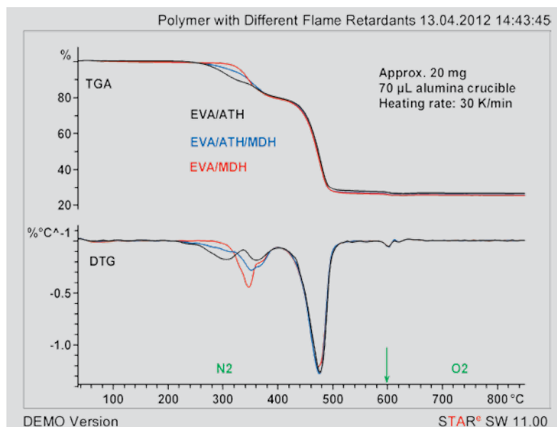
Figure 40. TGA analysis of EVA containing different flame retardants.
