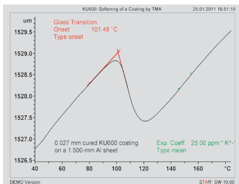
Figure 28. TMA measurement of a thin coating of cured KU600 to determine the softening temperature.
